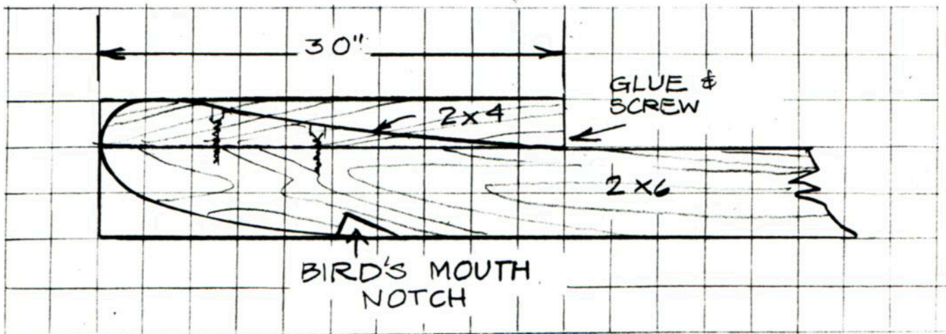
RAFTER TAIL PROFILE
